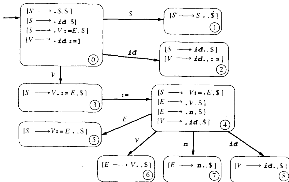
图5-8 例5.16中LR(1)项目集合的DFA
