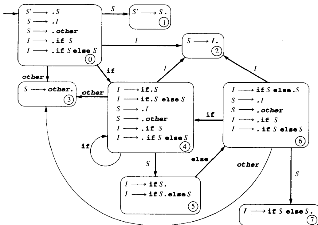
图5-6 例5.12中LR(0)项目集合的DFA
